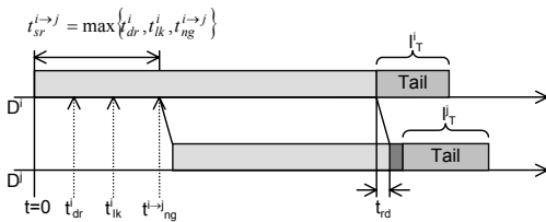
Figure 4: Relaying behaviour of a cut-through IS
